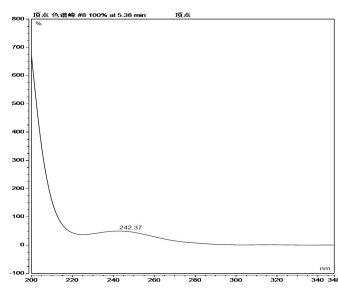
杀虫双
