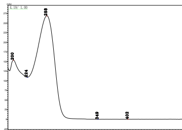
敌枯双
