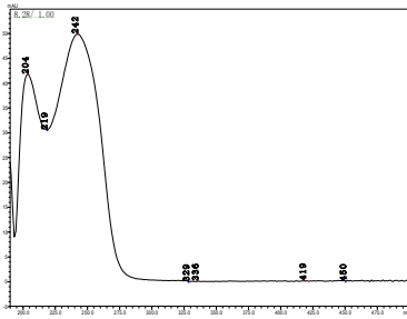
噻吡嘧磺隆
