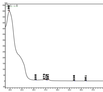
戊菌唑
