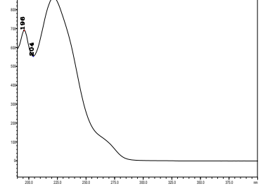
扑草净
